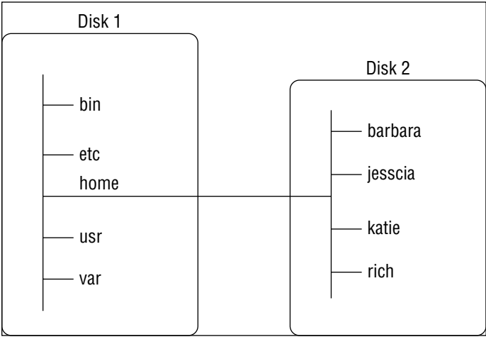
FIGURE 3-3 The Linux file structure
