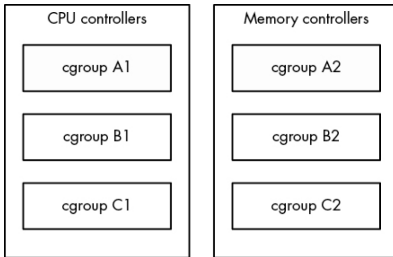
Figure 8-1: cgroups v1. A process may belong to one cgroup per controller.
